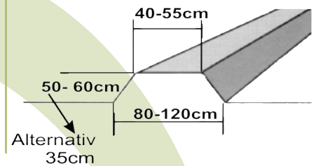
INDICATIVE DYKE DIMENSIONS
