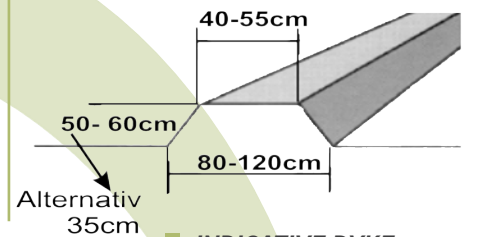
INDICATIVE DYKE DIMENSIONS
