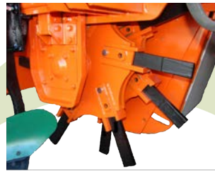
PATENTED ROTOR WITH SLOTS FOR BLADES AND PEG SUPPORT, CAPABLE OF BEING SHIFTED 3 TIMES, REINFORCED ROTORS WITH ANGLES
