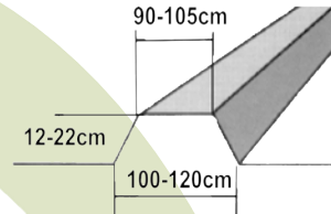
INDICATIVE DYKE DIMENSIONS
