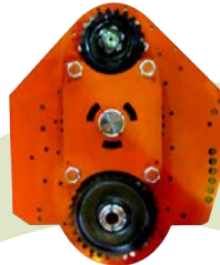
Lateral transmission with gears, Modul=6
