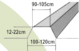
INDICATIVE DYKE DIMENSIONS
