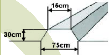
INDICATIVE DYKE DIMENSIONS
