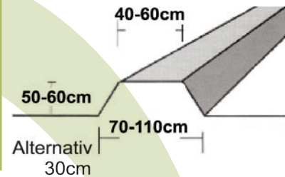
INDICATIVE DYKE DIMENSIONS
